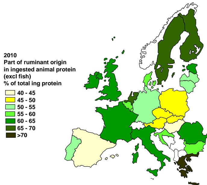
Figure S3. Share of ruminant products (milk, cheese, beef, mutton and goat meat) in total animal protein consumption (excluding fish and sea food) in 2010 2 .
