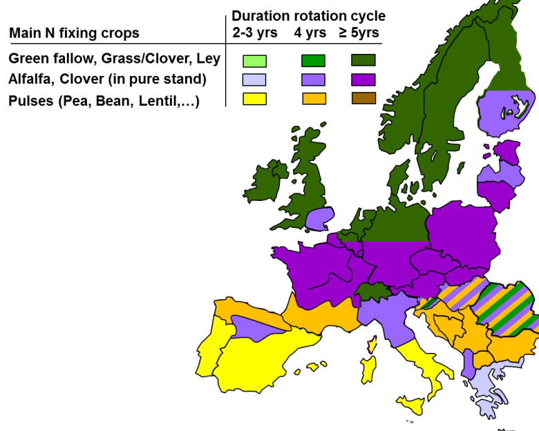
Figure S5. Tentative map of dominant crop rotations in organic cropping systems in Europe .
