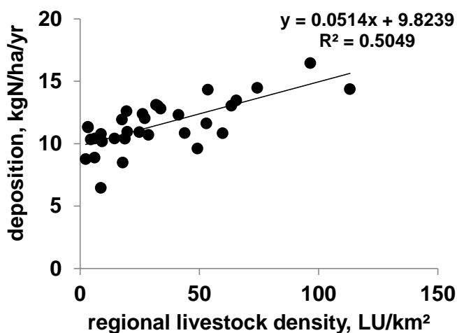
Figure S7. Relationship between atmospheric nitrogen deposition and livestock density for agricultural regions in France in 2006 84 .
