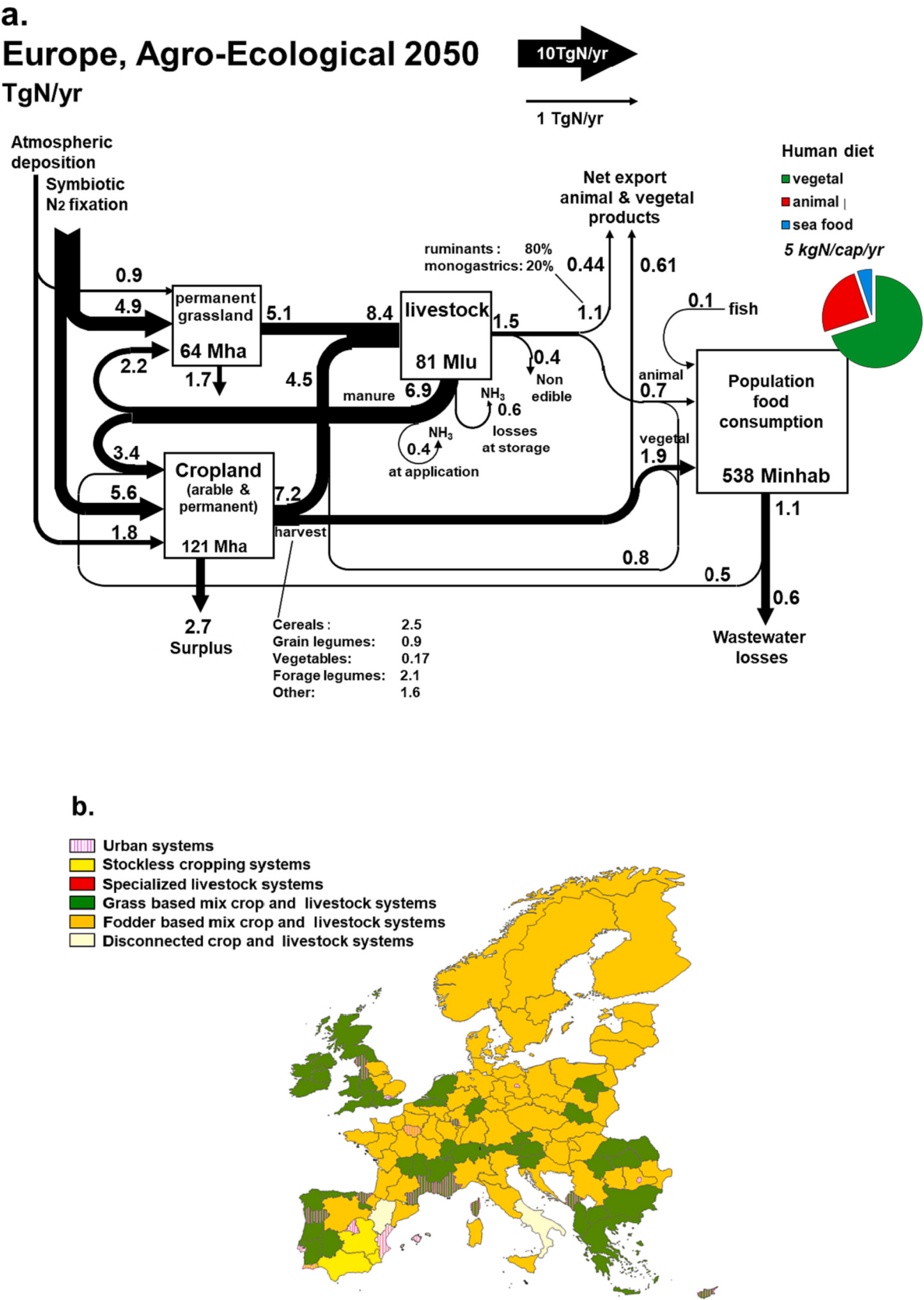
Fig. 6. a. GRAFS representation of N fluxes through the European agri-food system in 2050 in the Agro-Ecological scenario. b. corresponding distribution of the typological classes of regional agri-food systems.
