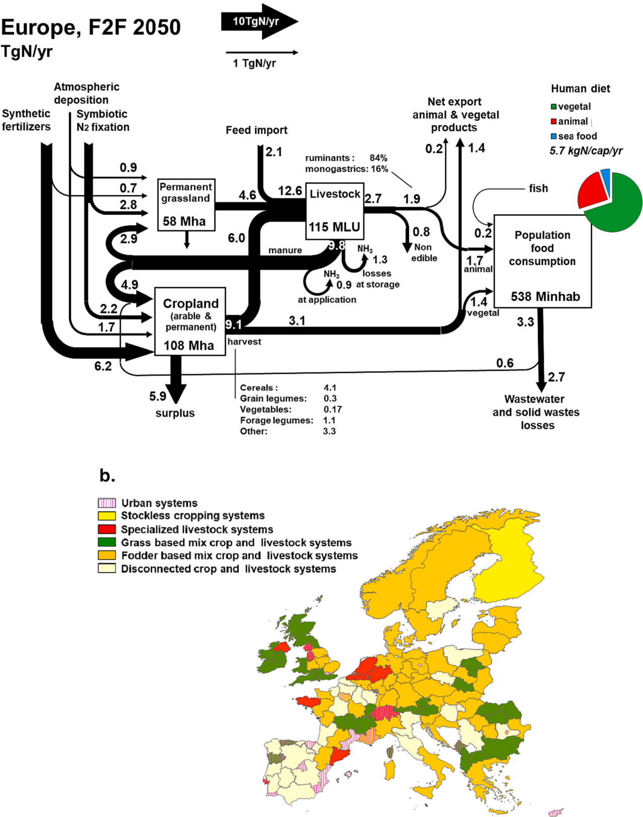
Fig. 7. a. GRAFS representation of N fluxes through the European agri-food system in 2050 in the F2F scenario. b. corresponding distribution of the typological classes of regional agri-food systems.
