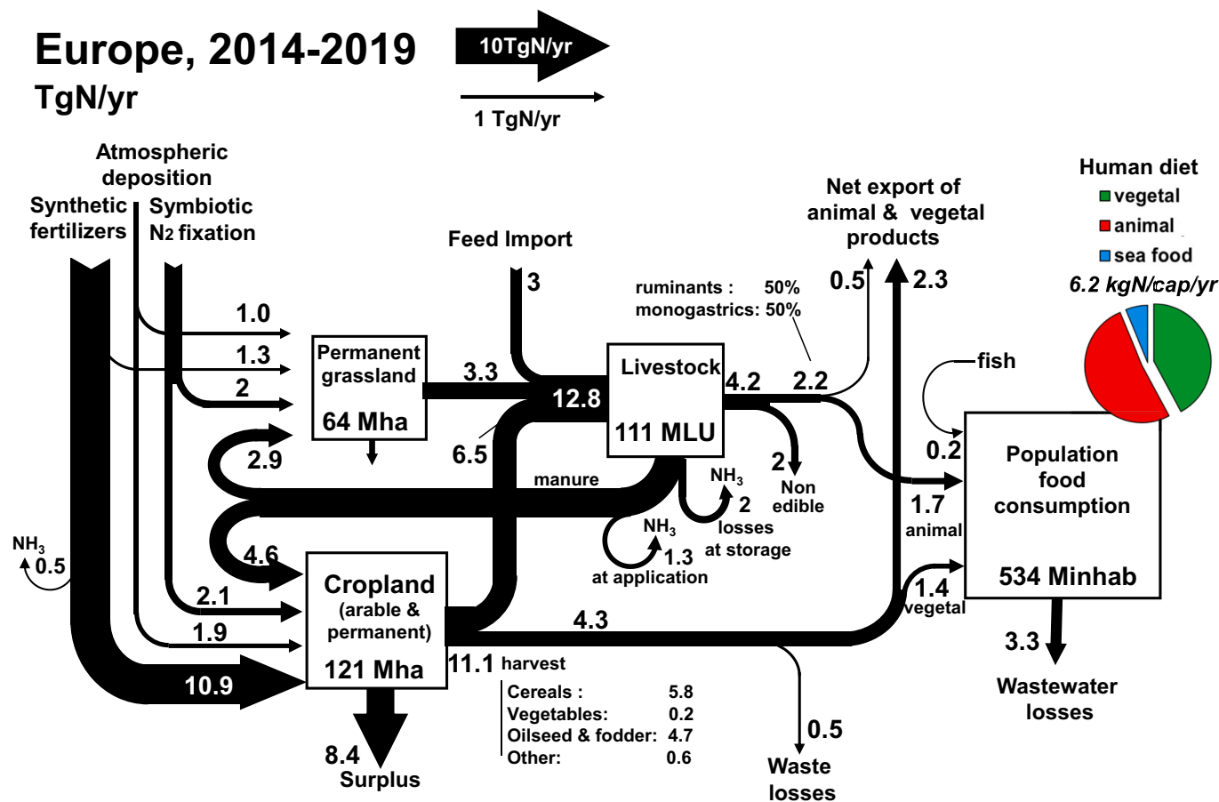
Fig. 1. Aggregated GRAFS representation of the current N fluxes through the European agri-food system in the period 2014–2019. This represents the sum of the fluxes for all 127 GUs considered across Europe. (“Surplus”, calculated as the balance of soil N inputs (after NH 3 volatilization at fertilizer and manure application) and harvest export, refers to losses through leaching and denitrification as well as to possible net increase of soil N pool).
