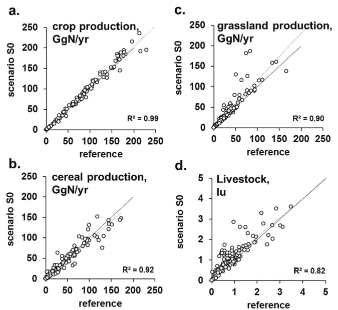
Fig. 5. Comparison of some major variables provided by the GRAFS accounting method for the Reference 2014–2019 situation of the European agri-food system at regional scale with the results of the scenario S0 established by the GRAFS Model for the same situation. (a.) Total cropland production; (b.) Cereal production; (c.) Permanent grassland production; (d.) Livestock units (1 LU = 85 kg N excretion/year). In the former approach, the variables in each region are directly derived from available statistical agricultural data, while in the latter approach they are calculated from total fertilization or available feed resources using the calibrated relationships discussed in Section 2.
